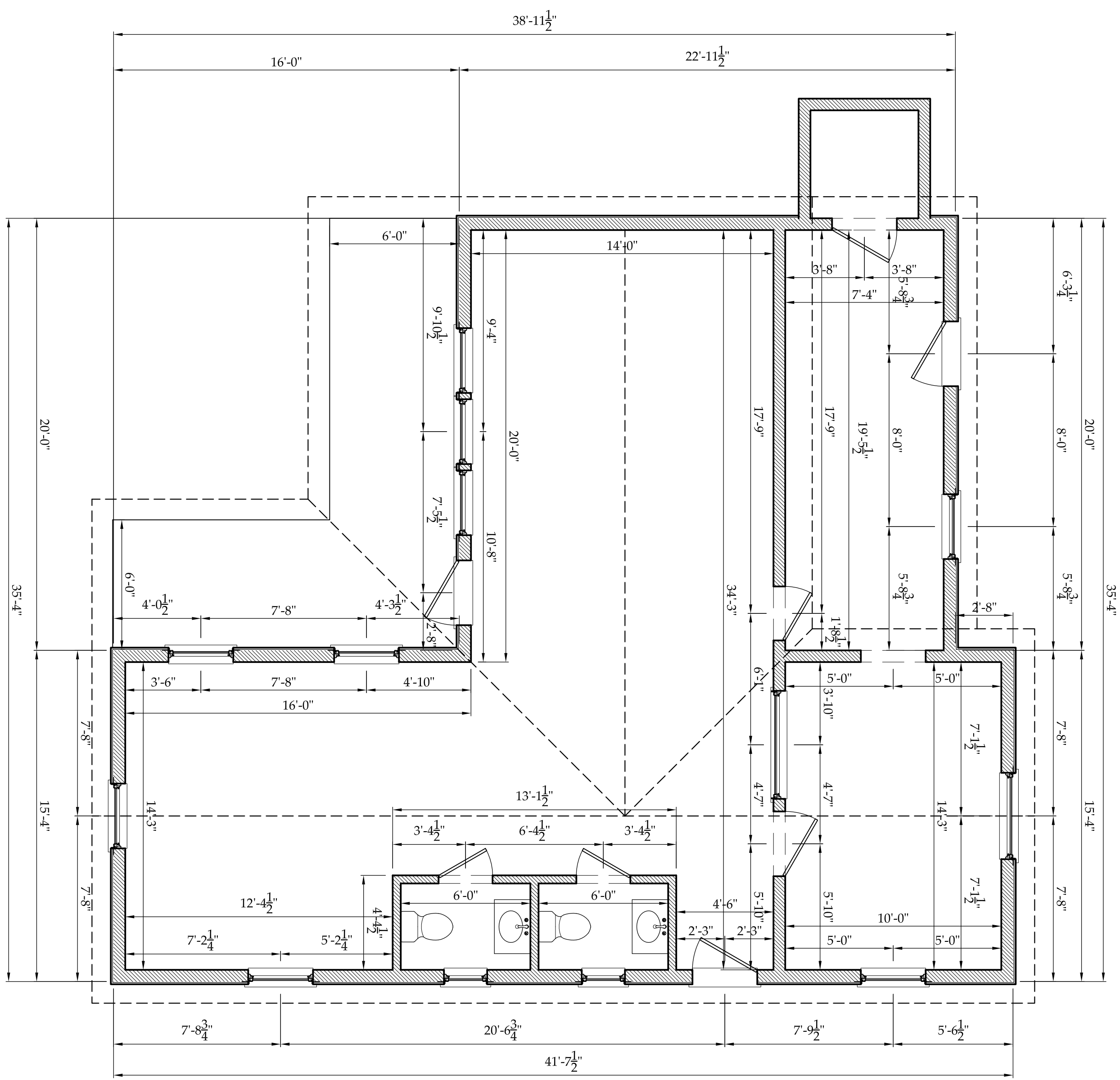
1 Main Level Floor Plan A1 SCALE: 1/4" = 1'-0" 0 4 8 16
